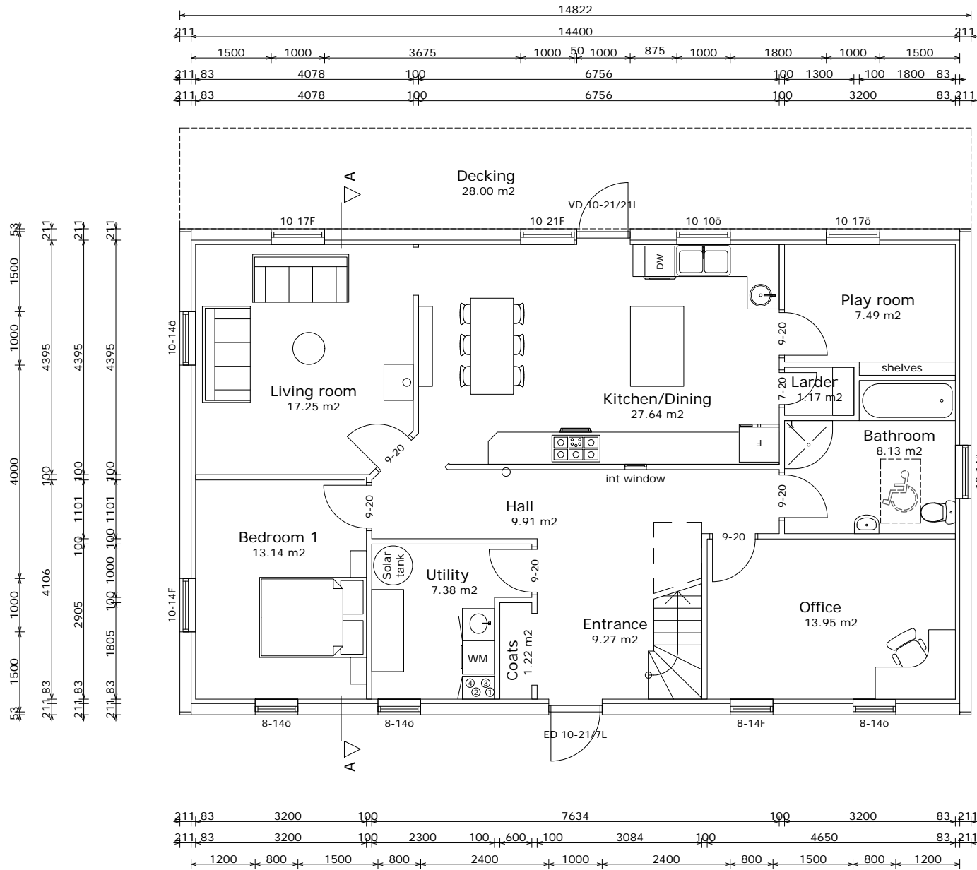
Ground floor 121.24 m 2
